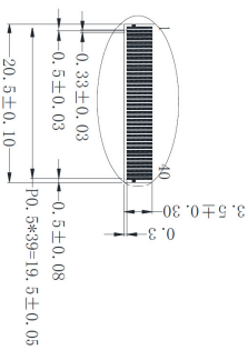
DETAIL A(2:1)
