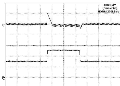
Plot 5 Line rejection at 1mA load Bottom: Input voltage (1V/div), Top: Output voltage (0.2V/div ac)
