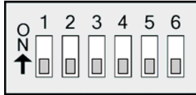
Figure B-13. RS-485 (2-wire) Half-Duplex DIP Switch Settings
