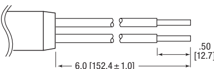
6" Wire Leads
