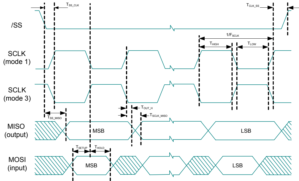
Figure 16. SPI Slave Mode 1 and 3
