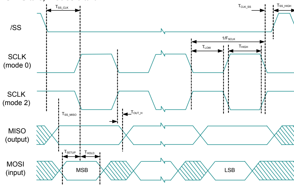
Figure 15. SPI Slave Mode 0 and 2
