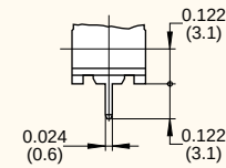
PCB Terminals RH Side with Location Pins 0.024 x 0.020 (0.6 x 0.5)
