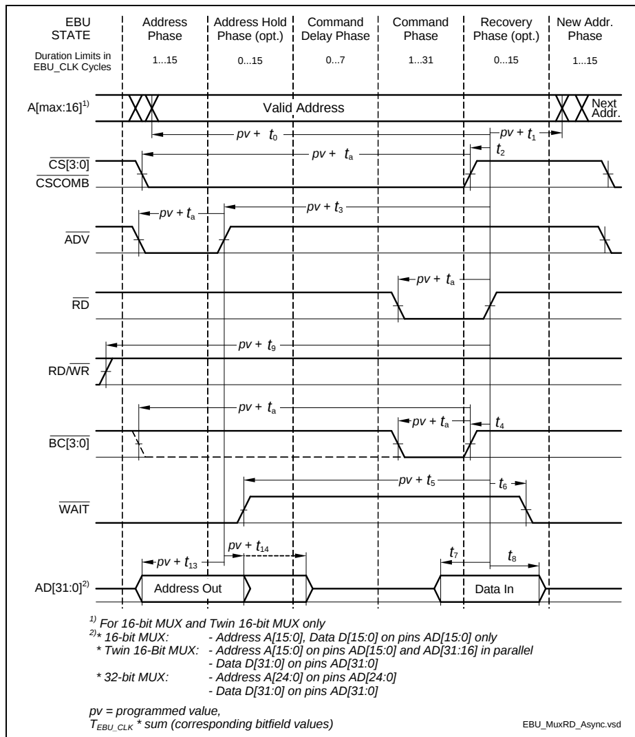
Figure 28 Multiplexed Read Access
