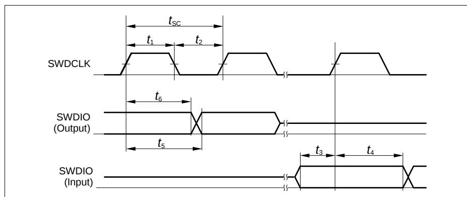
Figure 17 SWD Timing
