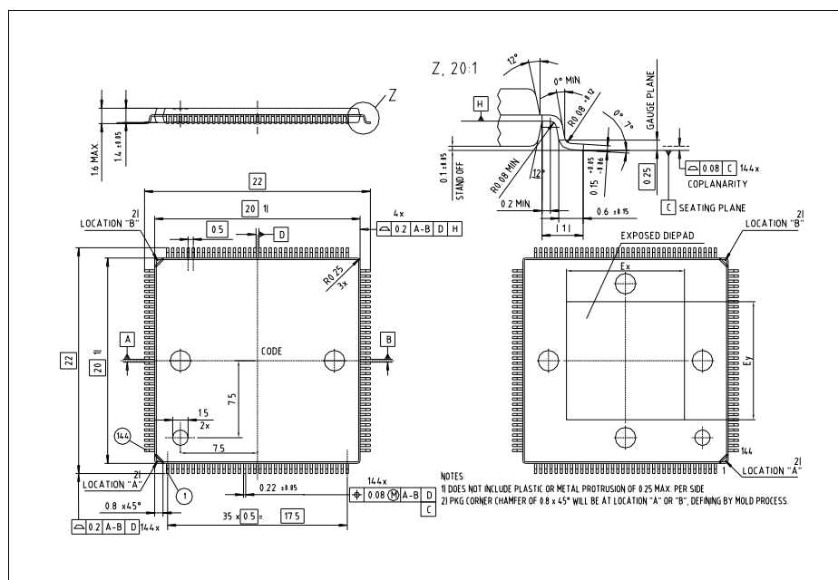
Figure 42 PG-LQFP-144-18 (Plastic Green Low Profile Quad Flat Package)
