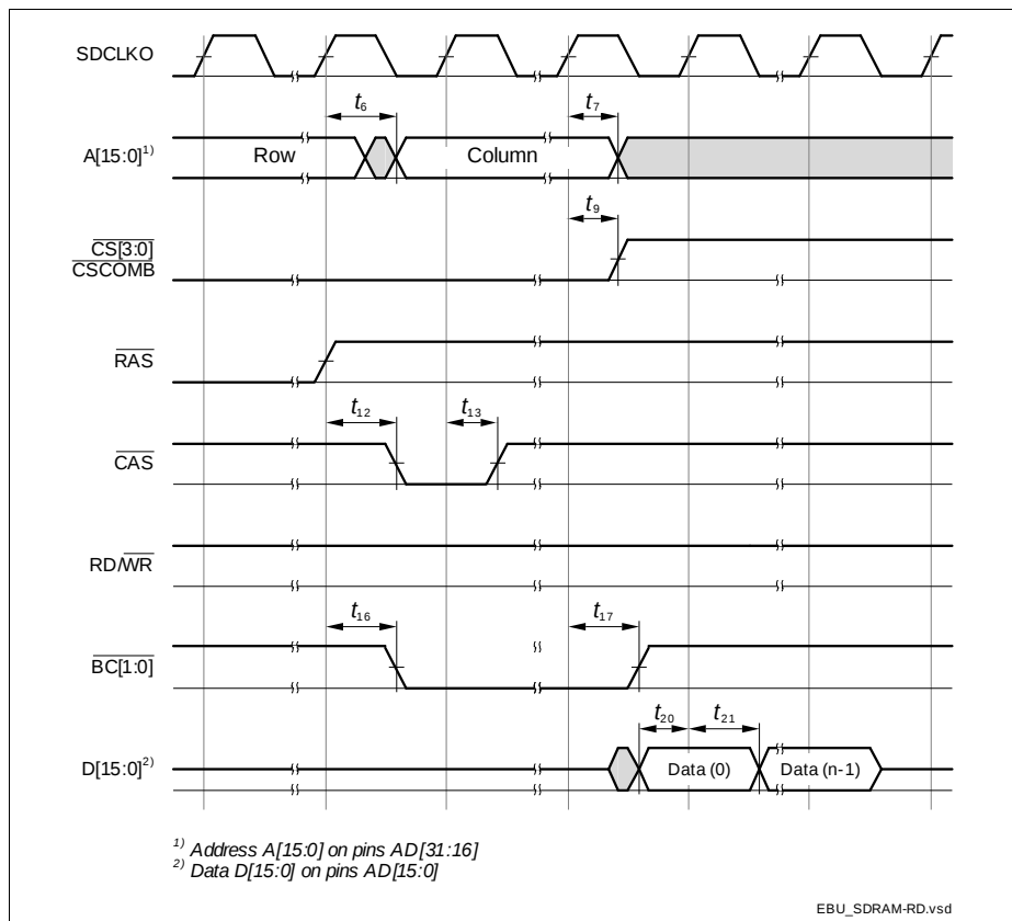
Figure 35 EBU SDRAM Read Access Timing
