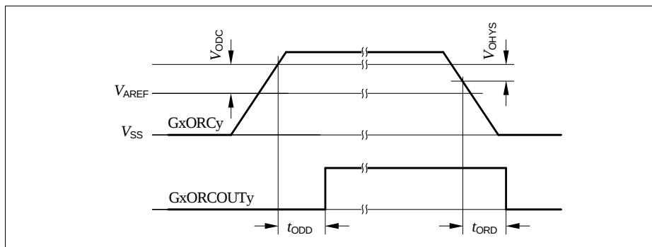
Figure 10 GxORCOUTy Trigger Generation
