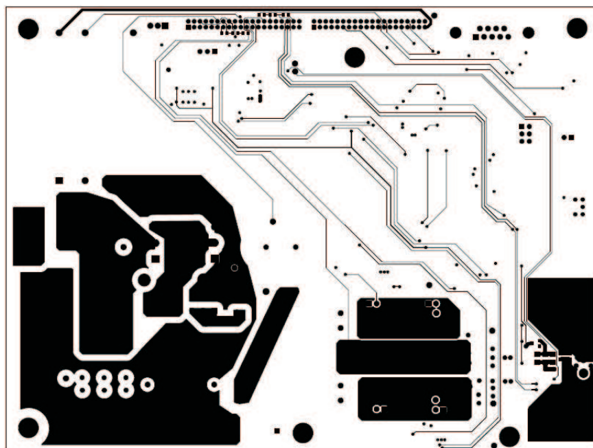
Figure 26. UCD3138LLCEVM-028 Bottom Copper (top view)
