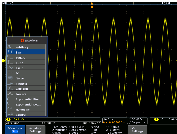
Waveform type selection in the integrated AFG.
