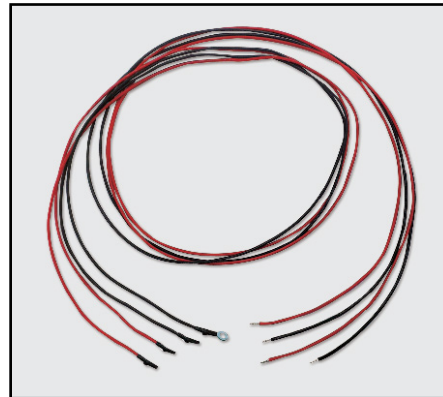
Model 2260-009: Test Lead Set for 250V and 800V models, two sets of red and black wires, 20AWG, 1.22m (48 in), stripped wires on one end and lugs on the other end.
