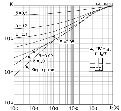
Figure 3: Thermal impedance
