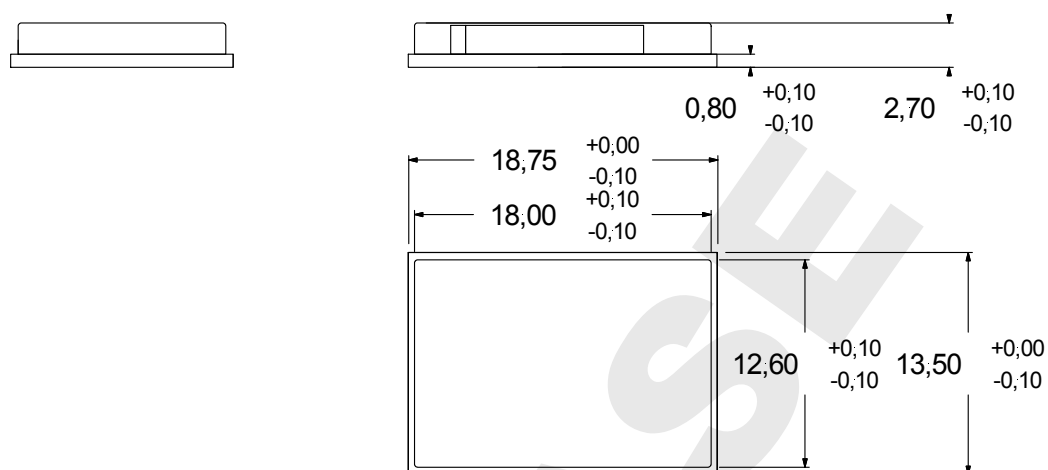
Figure 18.1 PAN1455 dimensions
