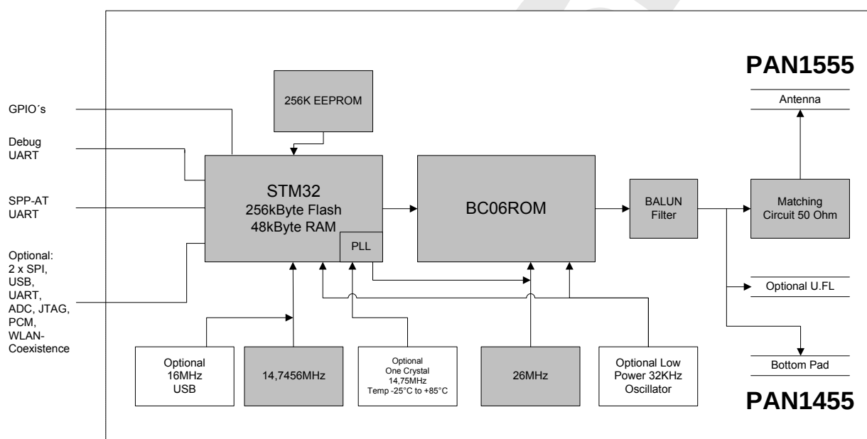
Figure 3.1 PAN1455/1555 Block-Diagram
