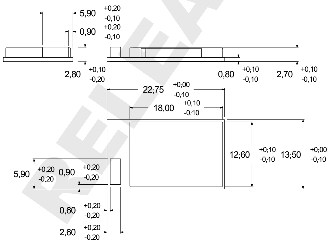
Figure 18.2 PAN1555 dimensions
