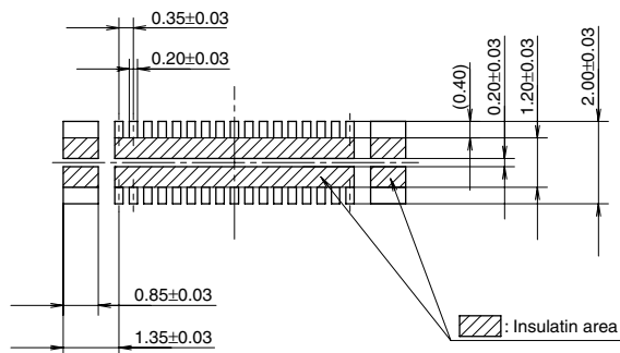
Recommended metal mask pattern
