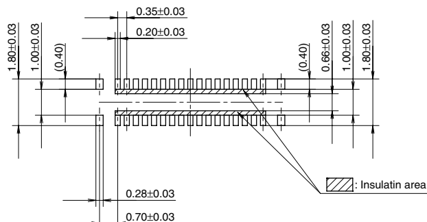
Recommended metal mask pattern
