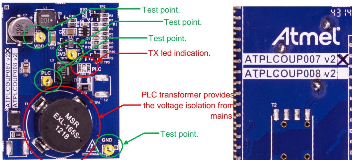
Figure 4-2. ATPLCOUP007v2.5 PLC Coupling board (top view).
