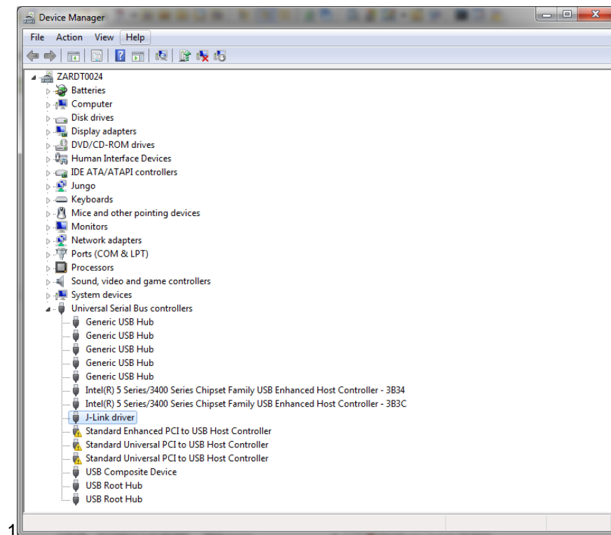
Figure 7-2. Device manager.
