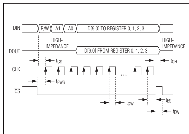
Figure 2. SPI Timing Diagram
