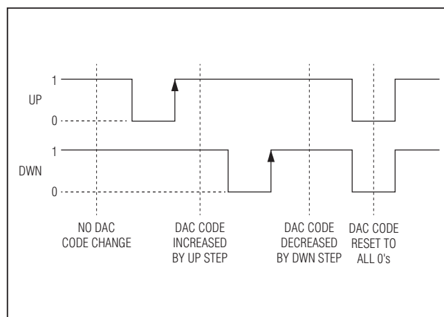
Figure 3. UP/DWN Control Diagram (MODE = 1)
