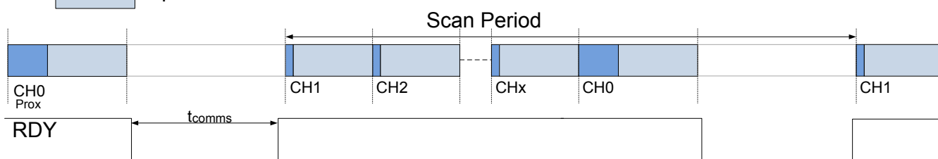
Figure 6.1 IQS333 Charge Sequence timing diagram in Boost Power mode.
