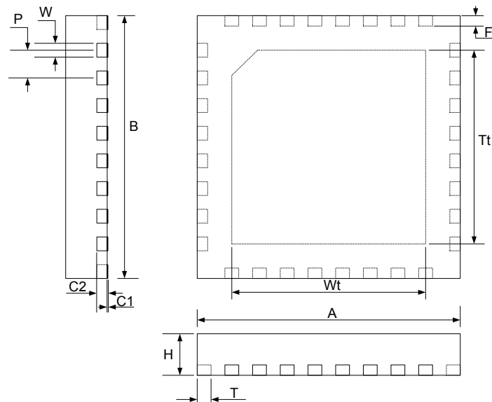
Figure 12.1 QFN(5x5) – 32 Package.
