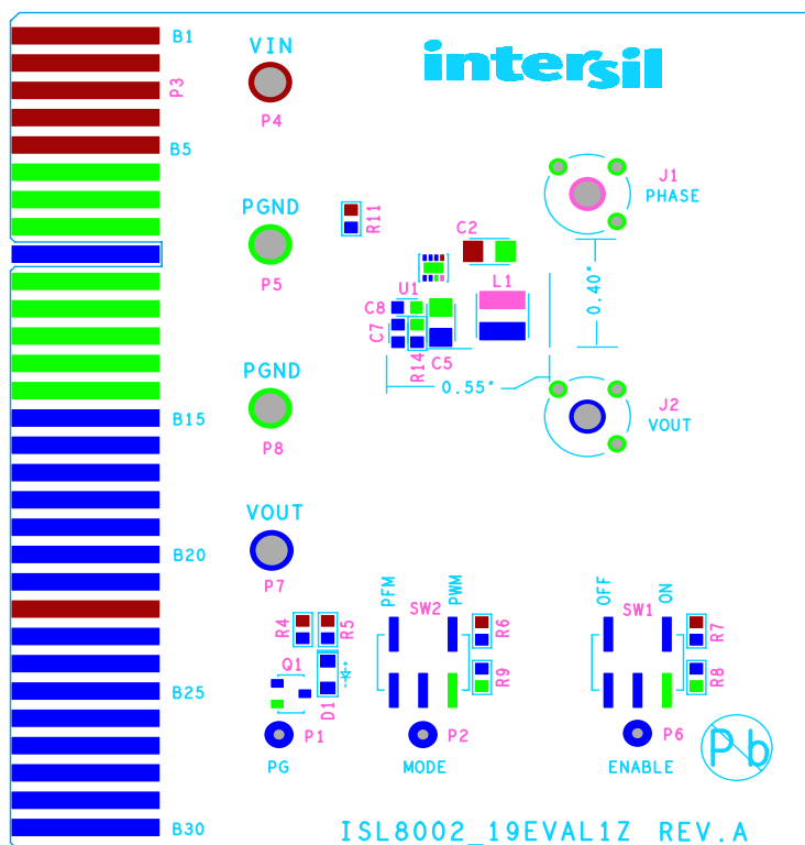
FIGURE 2. SILKSCREEN TOP
