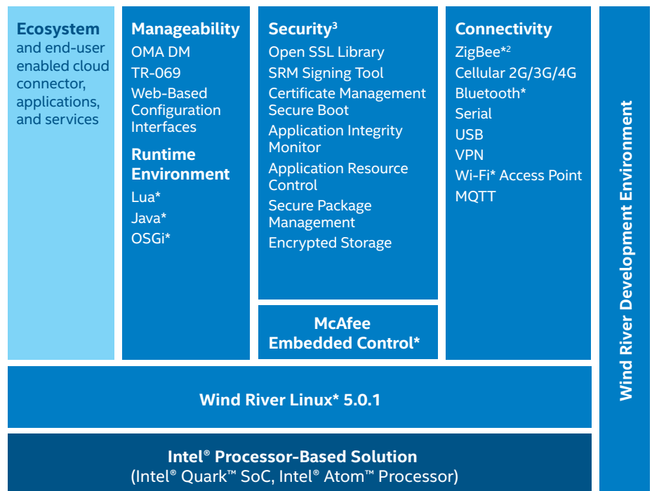
Figure 2.4 Intel® Gateway Solutions for IoT Software Stack.
