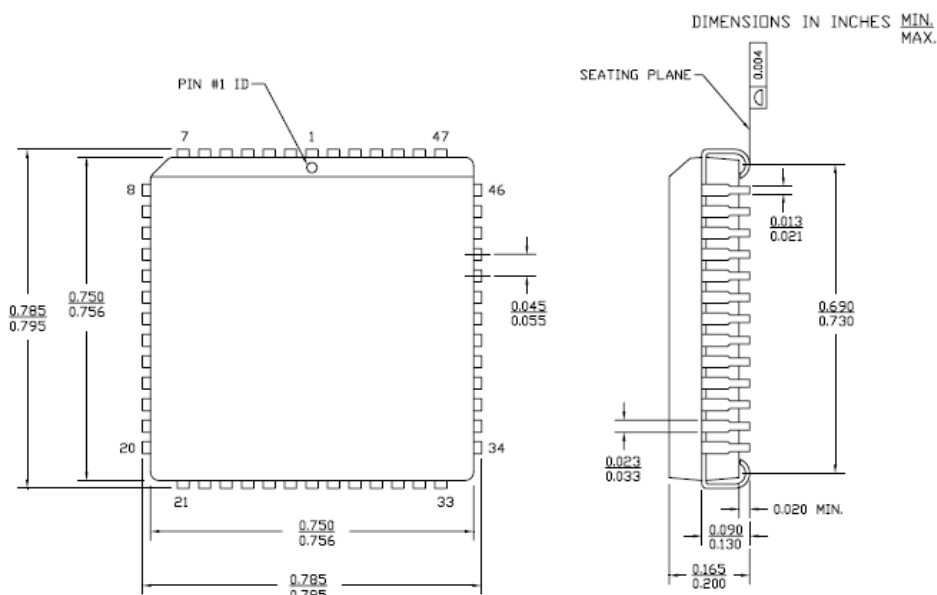
Figure 13. 52-pin PLCC (0.756 × 0.756 Inches) J52 Package Outline, 51-85004
