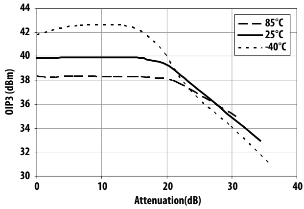
Figure 13. OIP3 vs Attenuation and Temperature at 1900MHz
