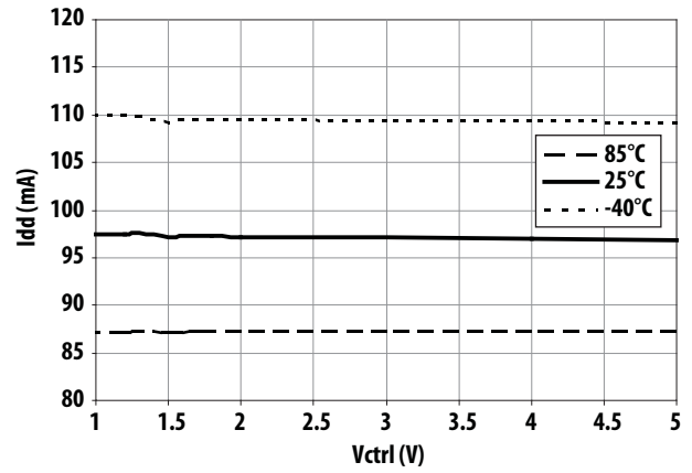
Figure 49. Current ( I_{dd} ) vs Control Voltage and Temperature
