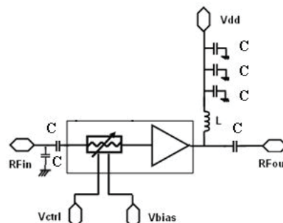
Figure 1. Simplified Schematic diagram
