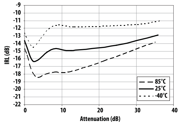
Figure 16. IRL vs Attenuation and Temperature at 1900MHz
