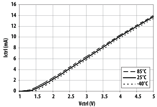
Figure 28. Current ( I_{ctrl} ) vs Control Voltage and Temperature
