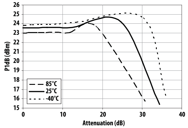
Figure 14. P1dB vs Attenuation and Temperature at 1900MHz
