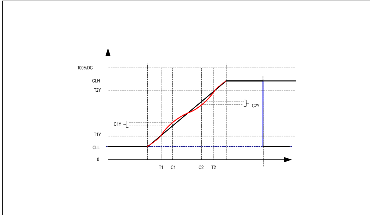
Figure 8. Linearization of the Output Characteristic
