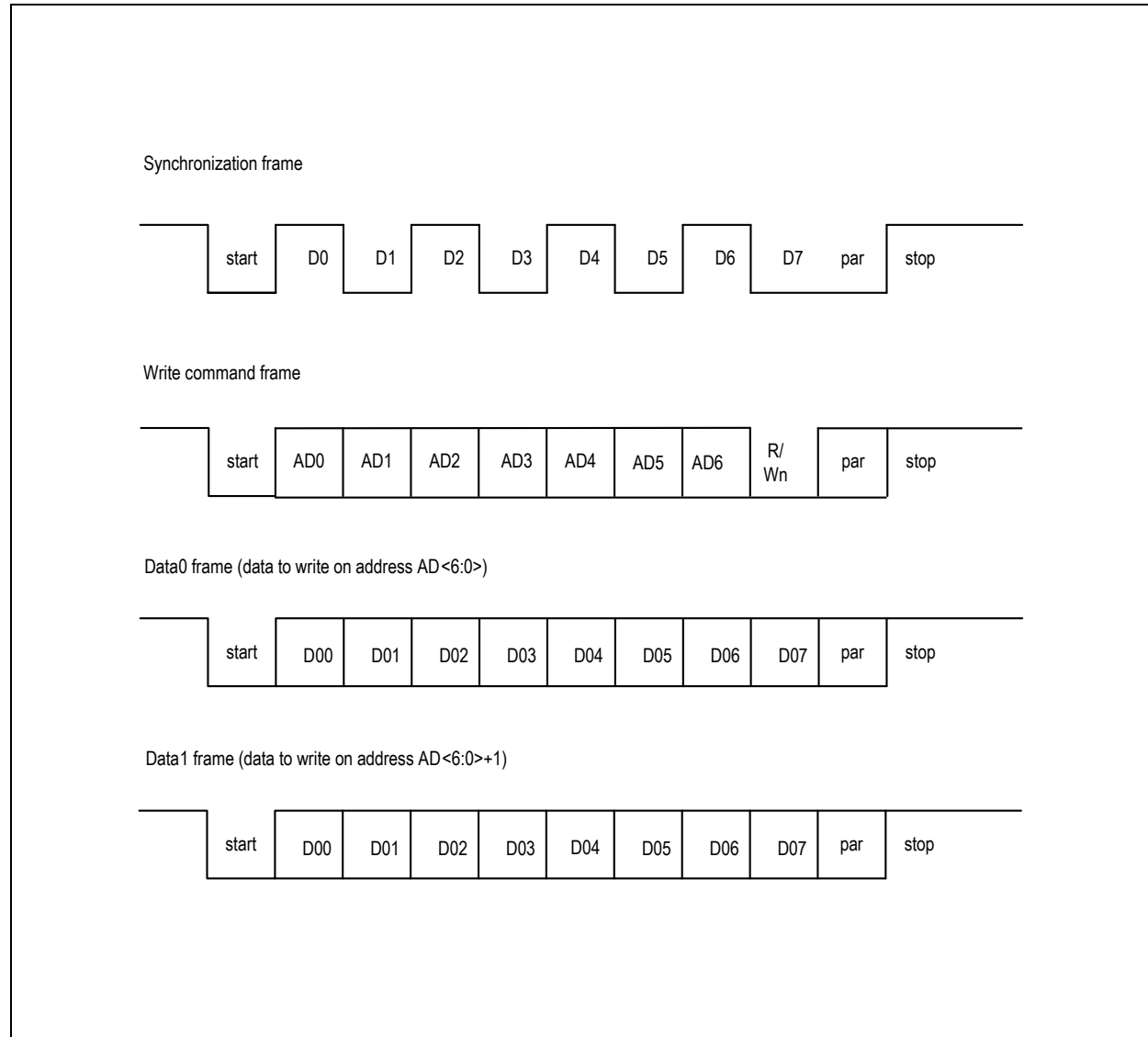
Figure 15. Full Write Command
