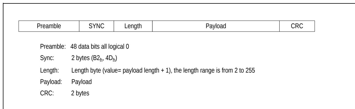
Figure 118: FeliCa Frame Format
