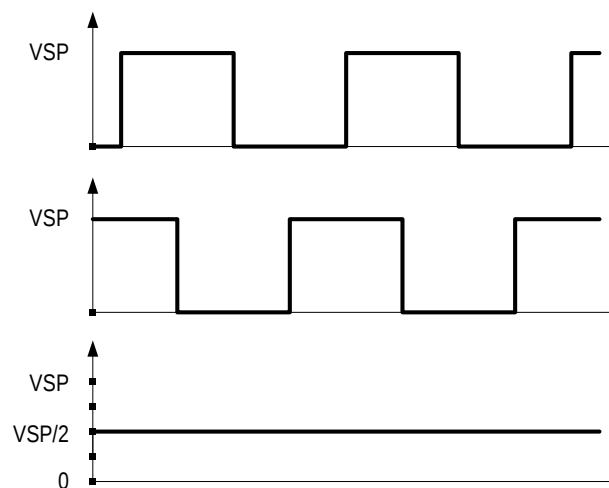
Figure 17: Phase Detector Inputs and Output in case of 90^\circ Phase Shift
