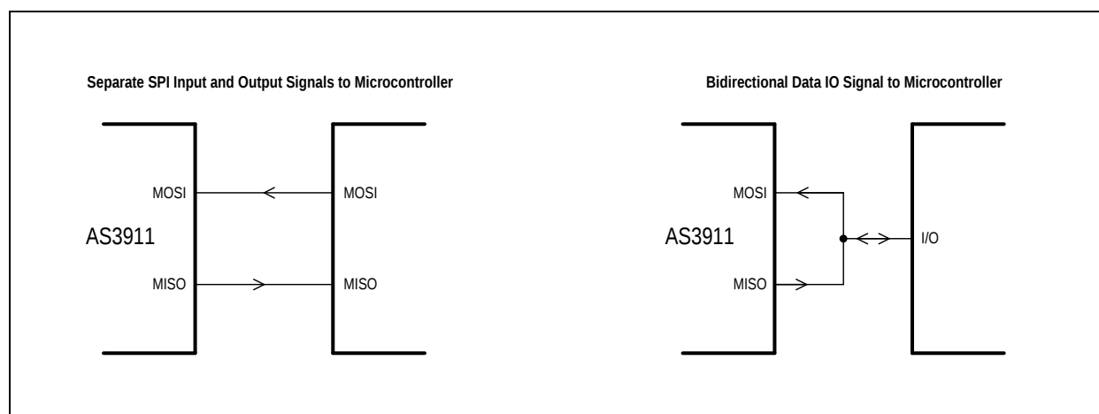
Figure 21: Signal to Microcontroller
