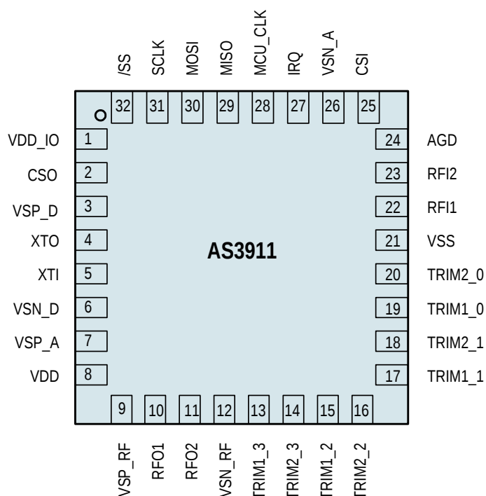
Figure 3: Pin Diagram
