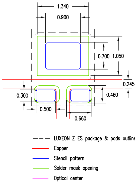
Figure 3. Solder pad layout for LUXEON Z ES.
