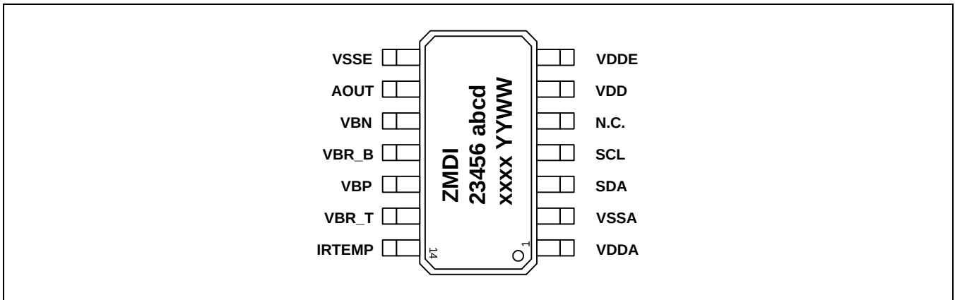
Figure 5.1 ZSSC3135 SSOP14 Pin Diagram
