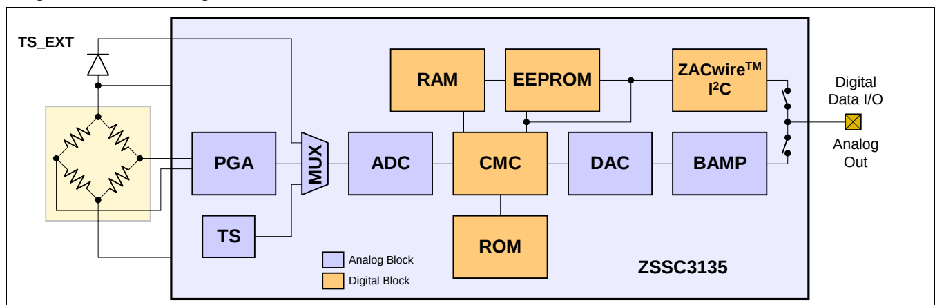
Figure 2.1 Block Diagram of the ZSSC3135
