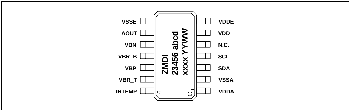
Figure 5.1 ZSSC3131 SSOP14 Pin Diagram
