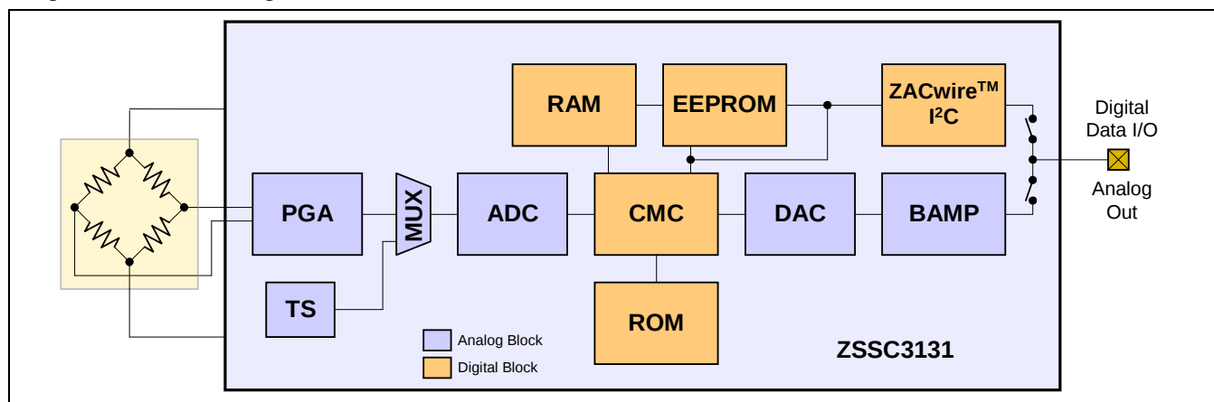
Figure 2.1 Block Diagram of the ZSSC3131
