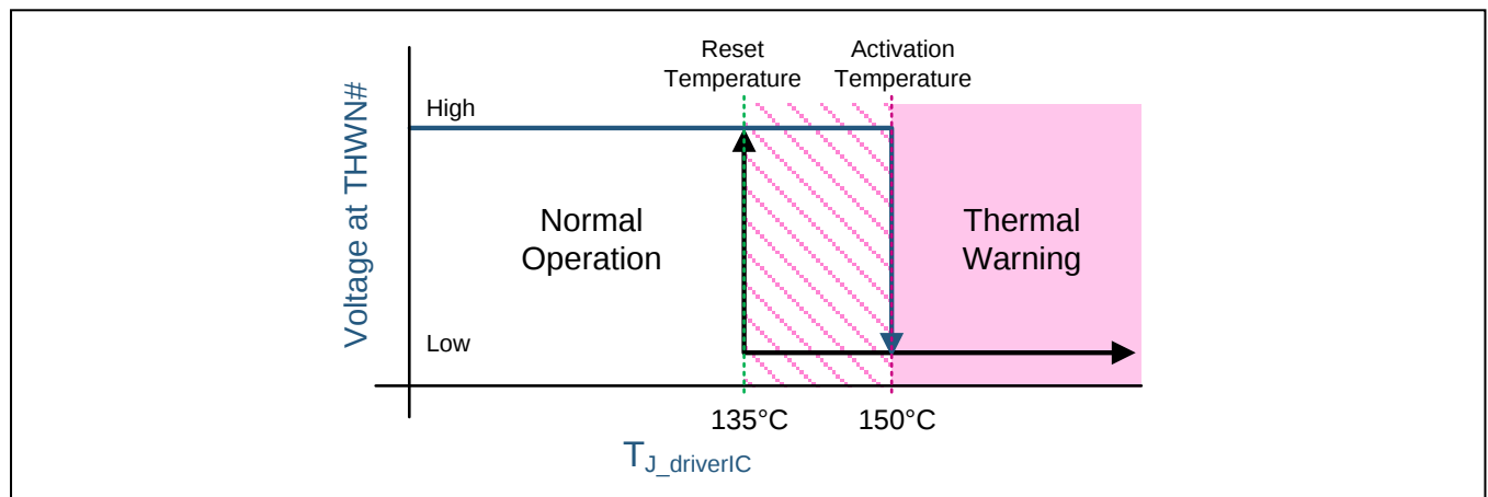
Figure 2.3 THWN# Operation
