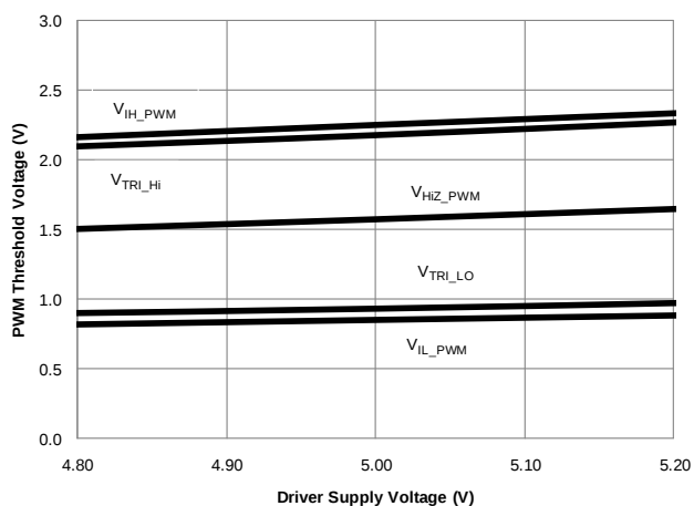
Figure 1.11 PWM Thresholds vs. Driver Supply Voltage
