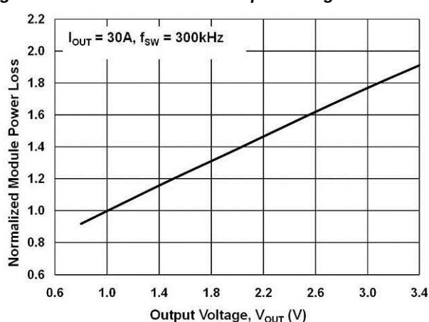
Figure 1.6 Power Loss vs. Output Voltage
