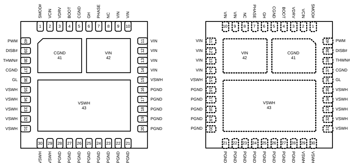
Bottom View
