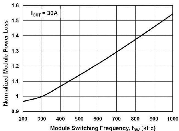
Figure 1.3 Power Loss vs. Switching Frequency
