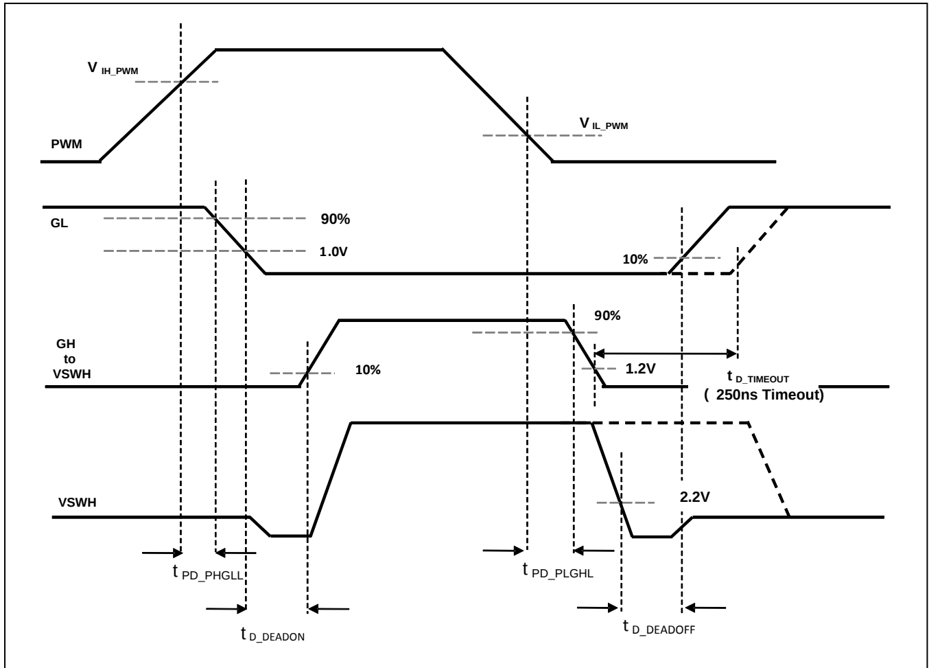
Figure 2.6 PWM Timing
