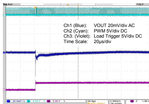
Figure 4.22 ZSPM1035C Open Loop Mode Plots with Capacitor Range #4
