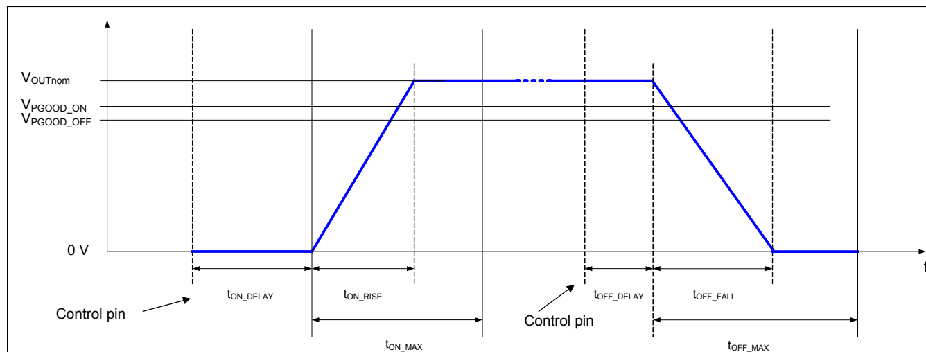
Figure 3.2 Power Sequencing
