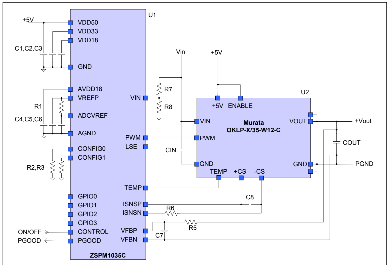
Figure 4.1 ZSPM1035C – Application Circuit with a 5V Supply Voltage
