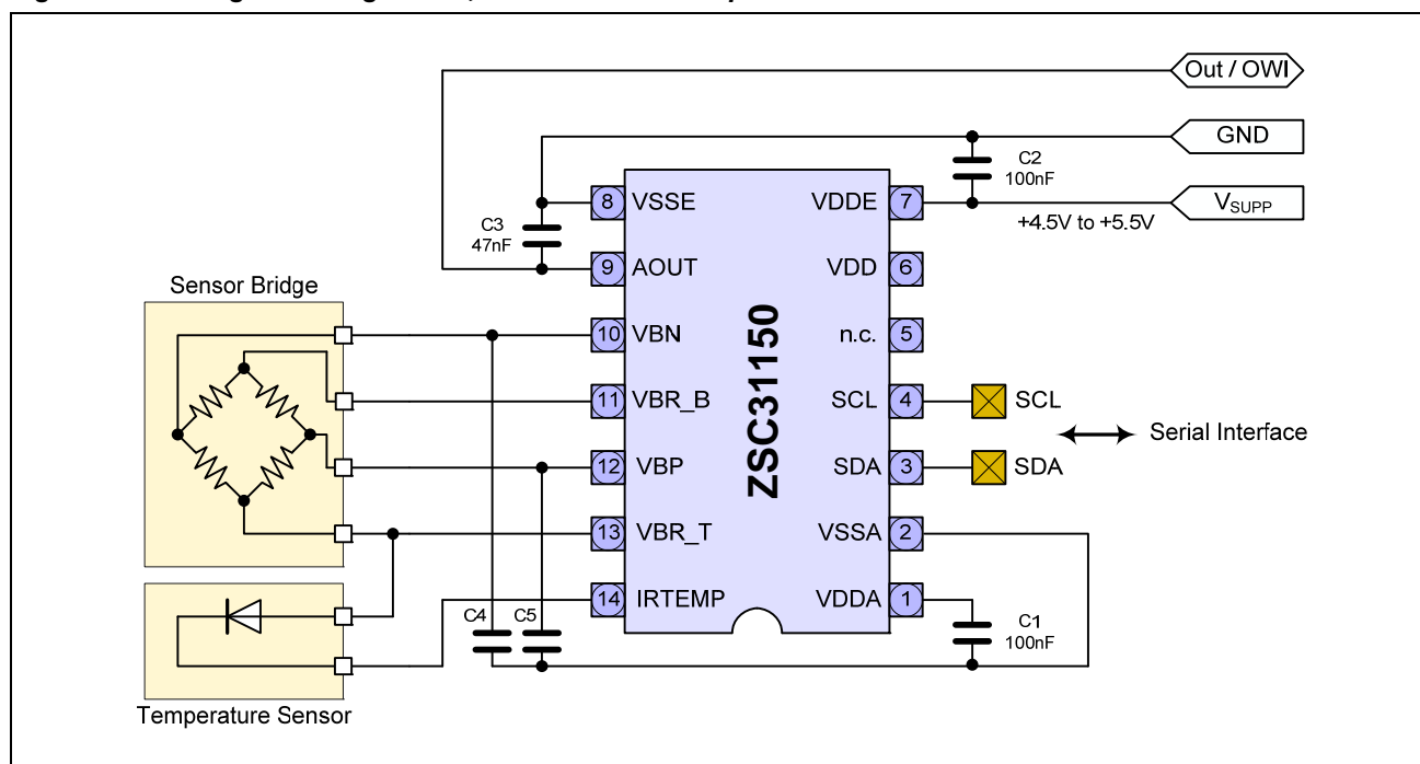
Figure 3.1: Bridge in Voltage Mode, External Diode Temperature Sensor
