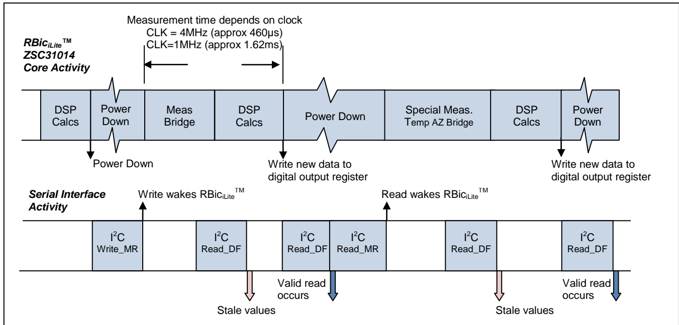
Figure 3.5 Sequence during Sleep Mode Using an I 2 C TM Write_MR to Wake Up (Typical Timing Values †† )
