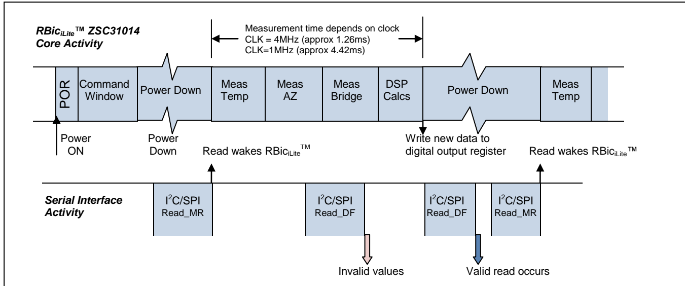
Figure 3.4 Power-on Sequence in Sleep Mode for I 2 C TM or SPI Read_MR (Typical Timing Values †† )
