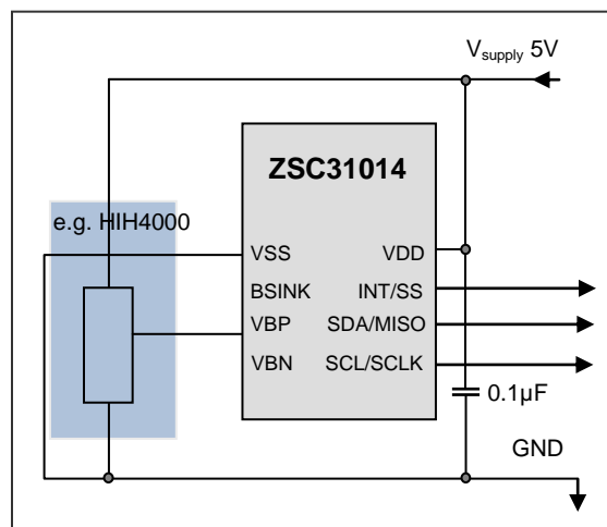
Figure 4.6 Half-Bridge Voltage Measurement with Internal Temperature Correction
