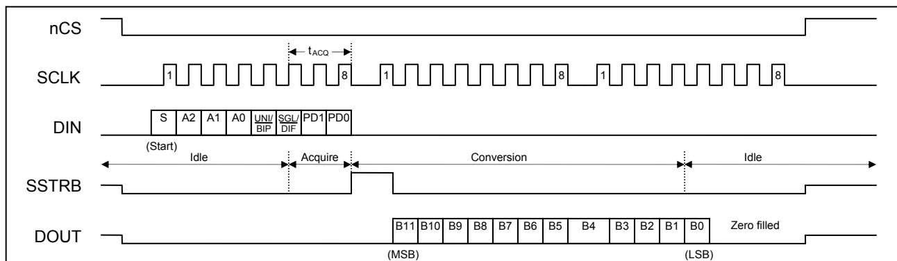
Figure 9: 24-Clock External Clock Mode Timing ( f_{SCLK} \leq 3.2\text{MHz} )
