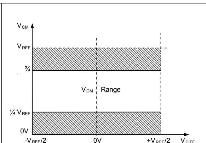
Figure 5: Input voltage range for bipolar mode
