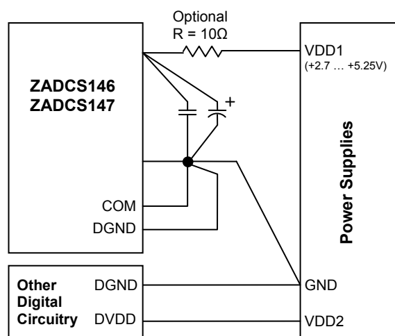
Figure 17: Optimal Power-Supply Grounding System
