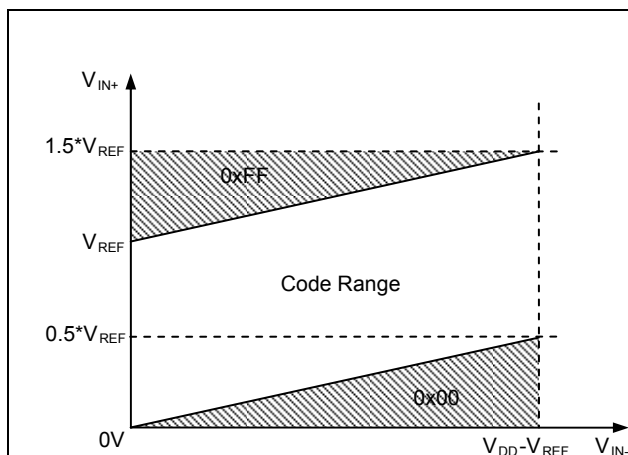
Figure 4: Input voltage range in unipolar mode
