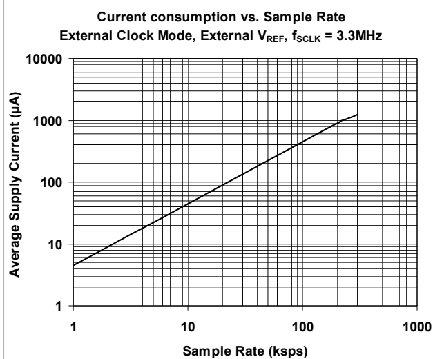
Figure 16: Supply Current versus Sampling Rate
