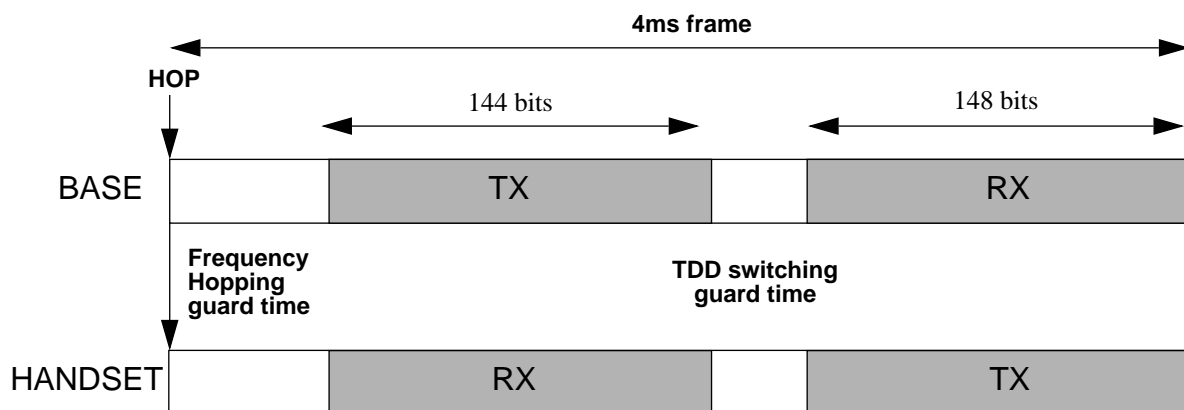
Figure 9. Basic Time Duplex Timing
