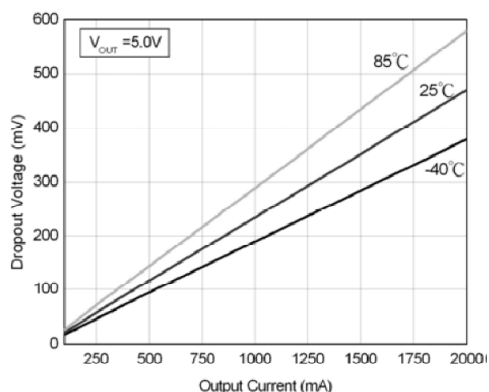
Fig. 12: Dropout Voltage at V_{OUT} = 5.0V
