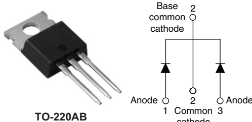
TO-220AB
