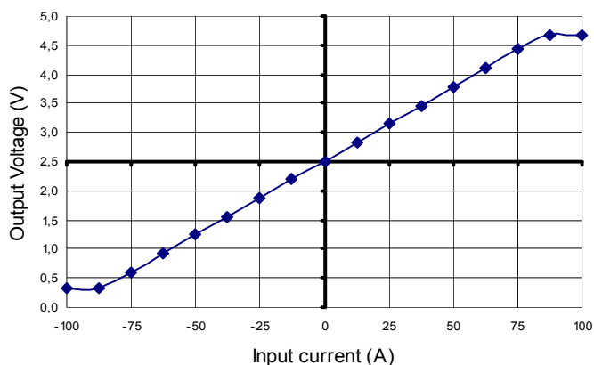
Saturation Characteristic
