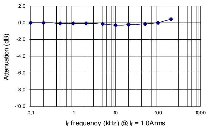
Frequency Characteristic
