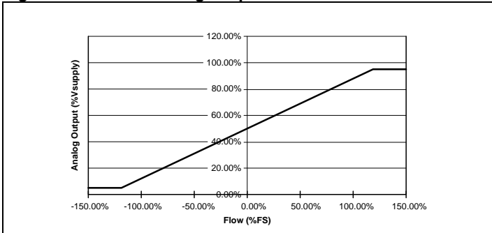
Figure 2. Nominal Analog Output
