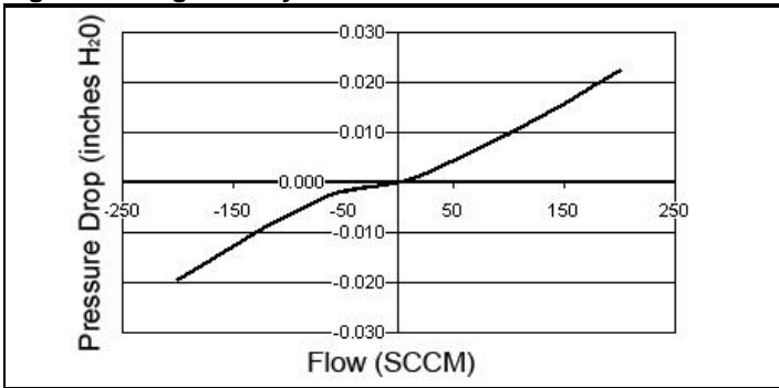
Figure 6. Long Port Style Flow vs Pressure
