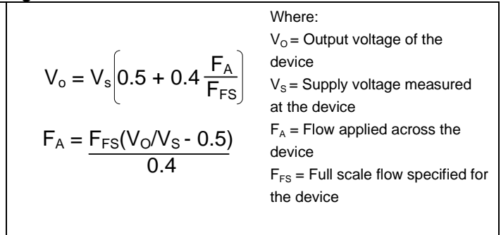
Figure 3. Ideal Transfer Function
