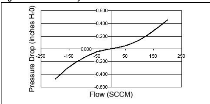
Figure .7 Short Port Style Flow vs Pressure
