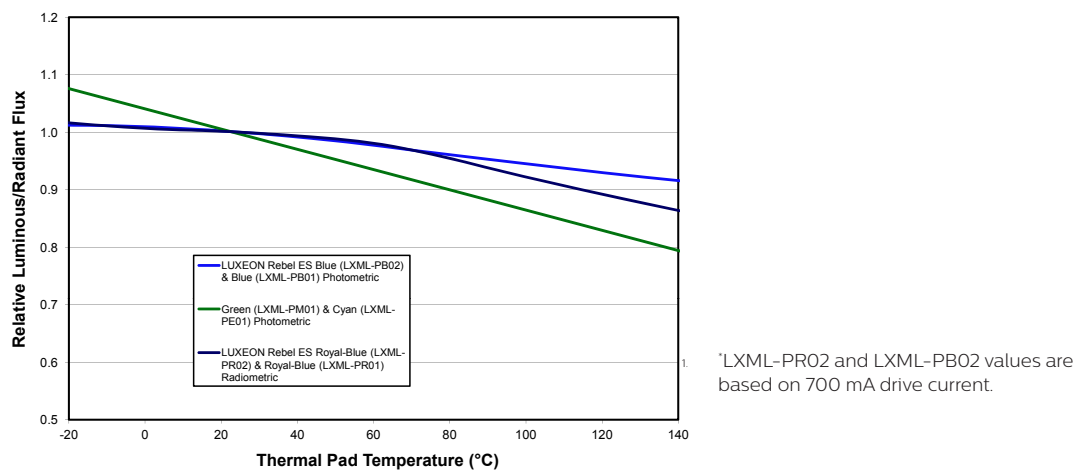
Figure 7. Relative light output vs. thermal pad temperature for green, cyan, blue and royal blue.
