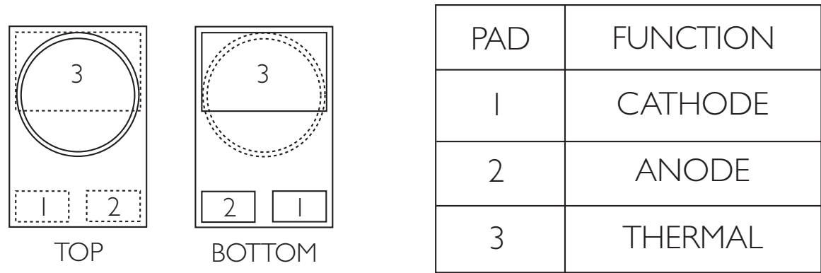
Figure 3. Solder pad layout.
