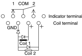
Latching
