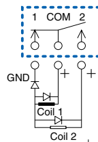
Latching
