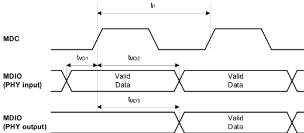
Figure 32. MDC/MDIO Timing
