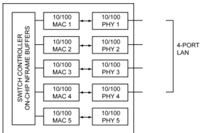
Figure 3. Standalone Switch
