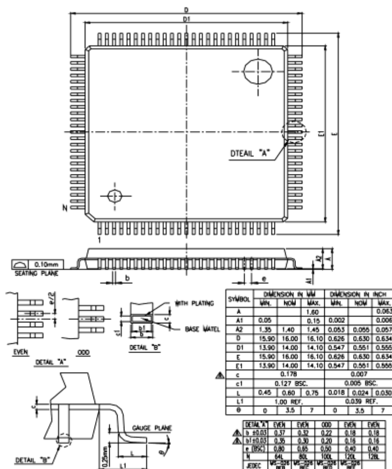
128-Pin LQFP Package
