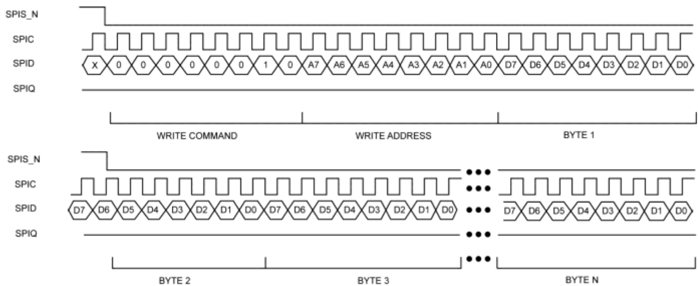
Figure 17. SPI Multiple Write
