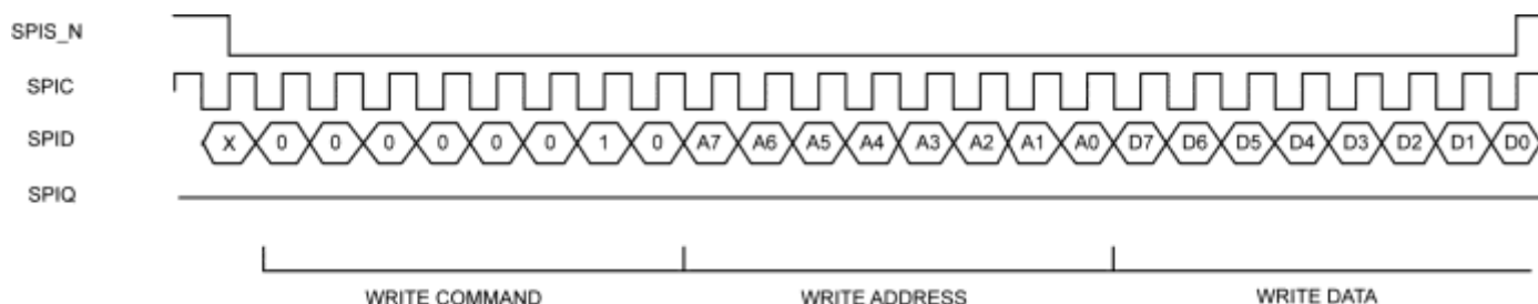
Figure 15. SPI Write Data Cycle
