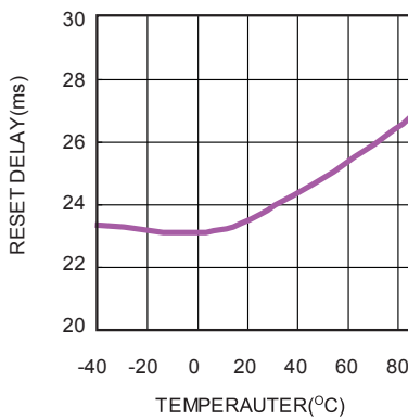
Reset Delay vs. Temperature ( C_{DELAY}=open )
