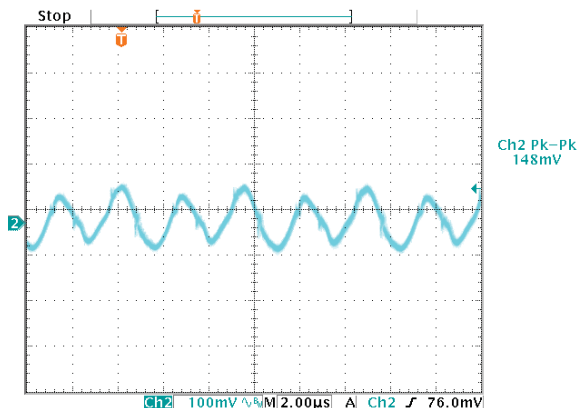
Ripple and Noise Waveform (Vin=48V Iout=16A)
