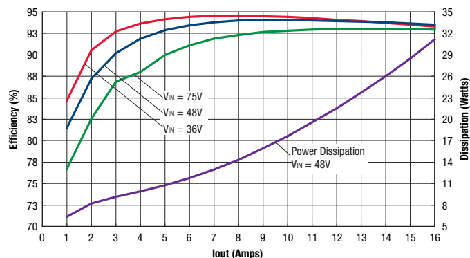
Efficiency and Power Dissipation @ Ta = +25°C
