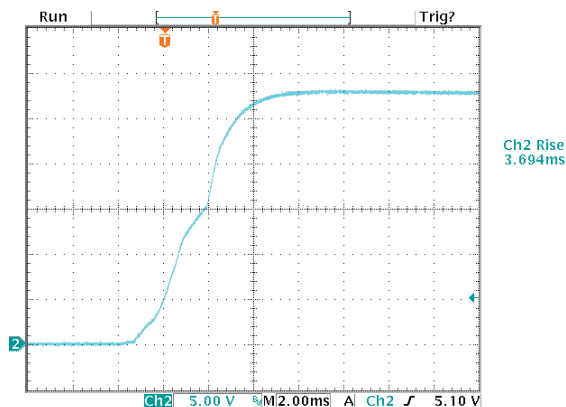
Enable Start-up (Vin=48V Iout=0A)
