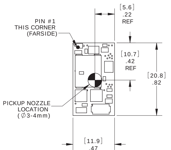
PICK & PLACE PICKUP (P/U)
