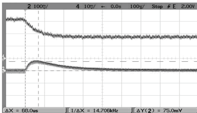
Step Load Transient Response (V IN =24V, V OUT =1.5V, Load=0, I OUT =3A to 1.5A) Trace 2=V OUT , 100 mV/div. Trace 4=I OUT , 1A/div.
