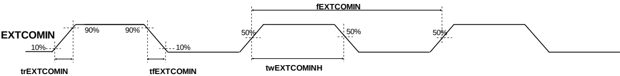
EXTCOMIN signal
