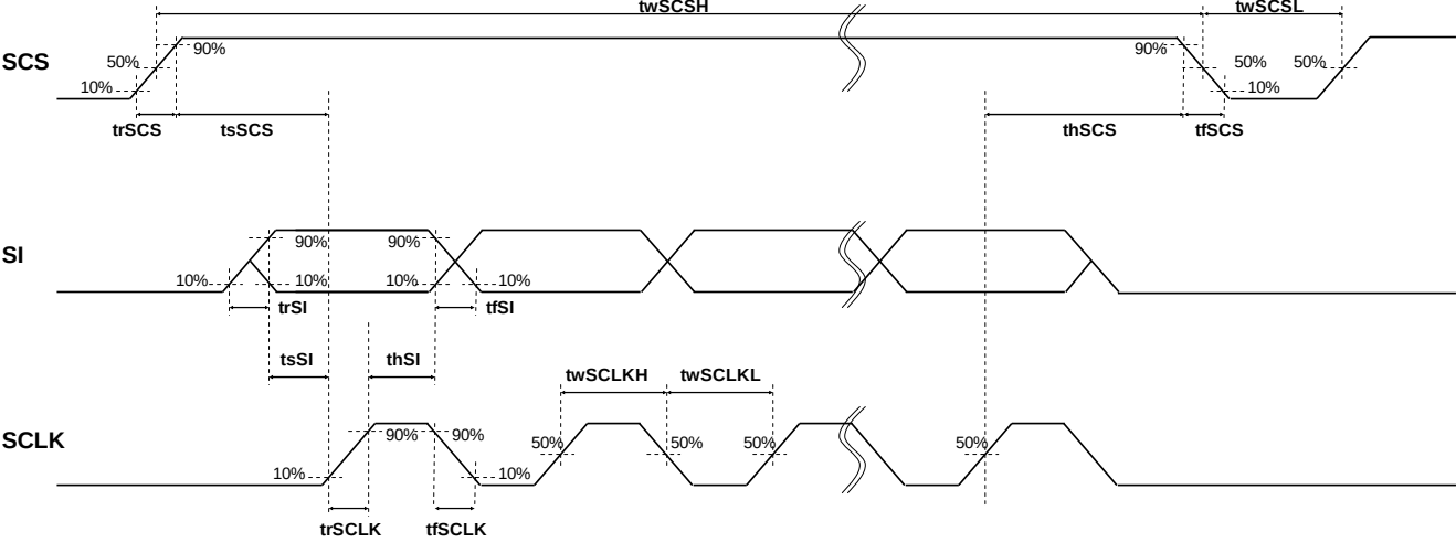
SCS, SI, SCLK signal
