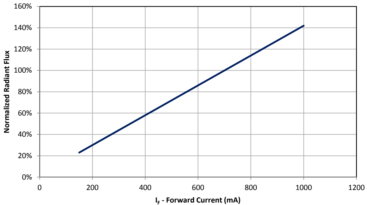
Figure 8: Typical normalized radiant flux vs. forward current @ T_C = 25^\circ\text{C}
