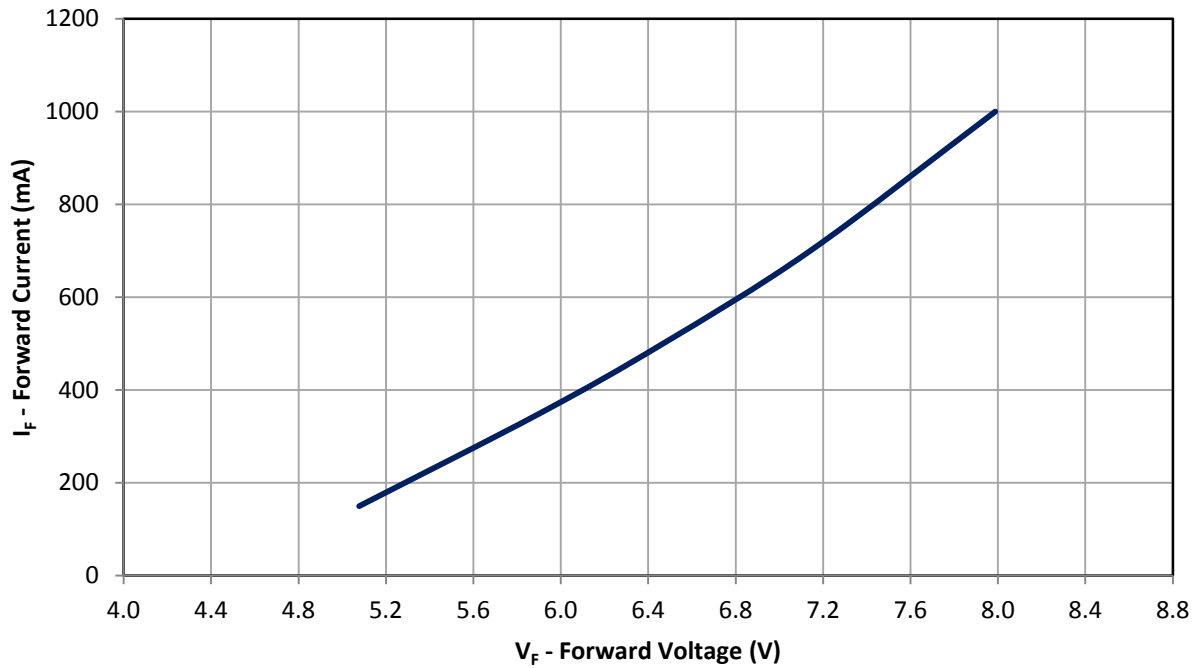
Figure 10: Typical forward current vs. forward voltage @ T_C = 25^\circ\text{C}
