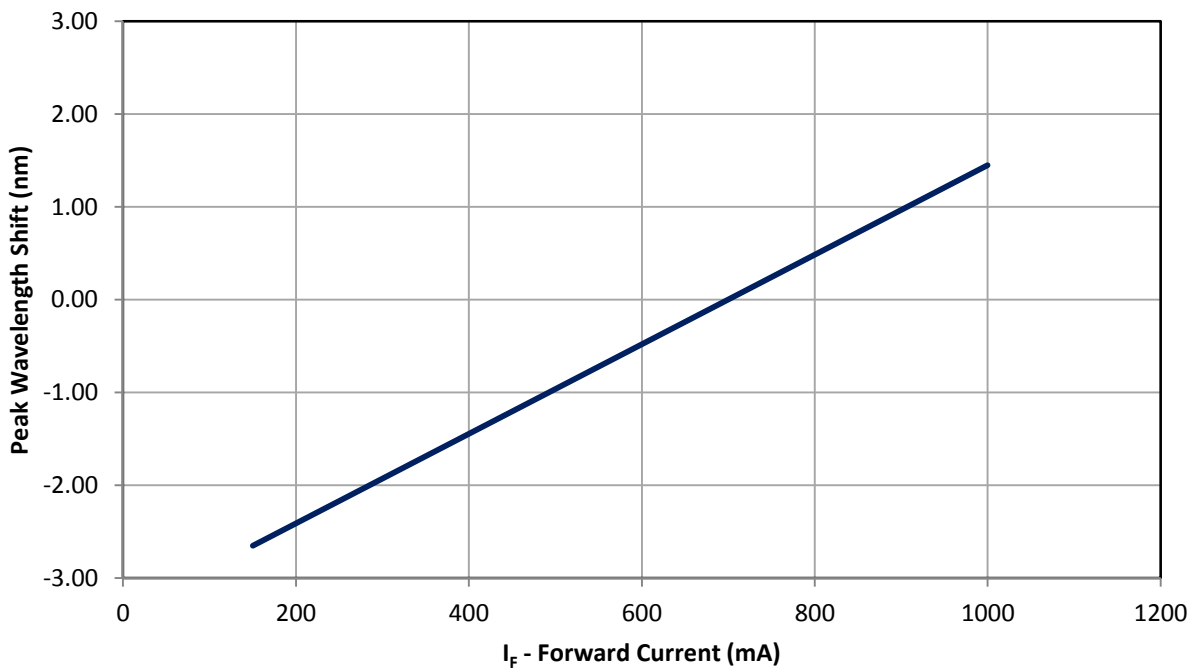
Figure 6: Typical peak wavelength shift vs. forward current @ T_c = 25^\circ\text{C}
