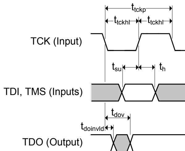
Figure 6.10 JTAG Timing
