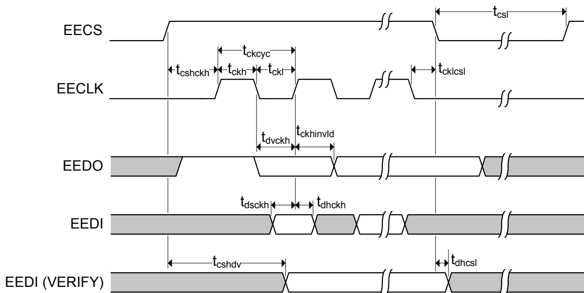
Figure 6.5 EEPROM Timing
