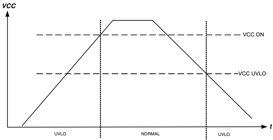
Fig. 14 - V_{CC} Under Voltage Lockout
