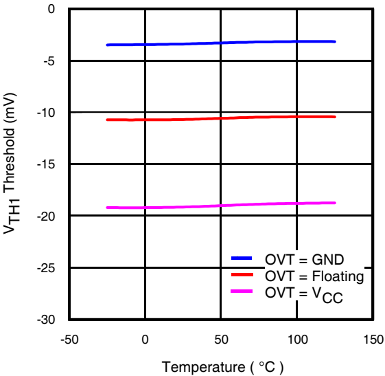
Fig 3. V_{\text{TH1}} vs. Temp.
