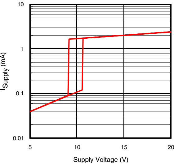
Fig 1. Supply Current vs. Supply Voltage
