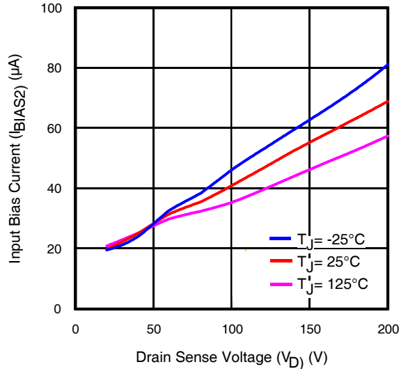
Fig 10. Input Bias Current vs. V D .
