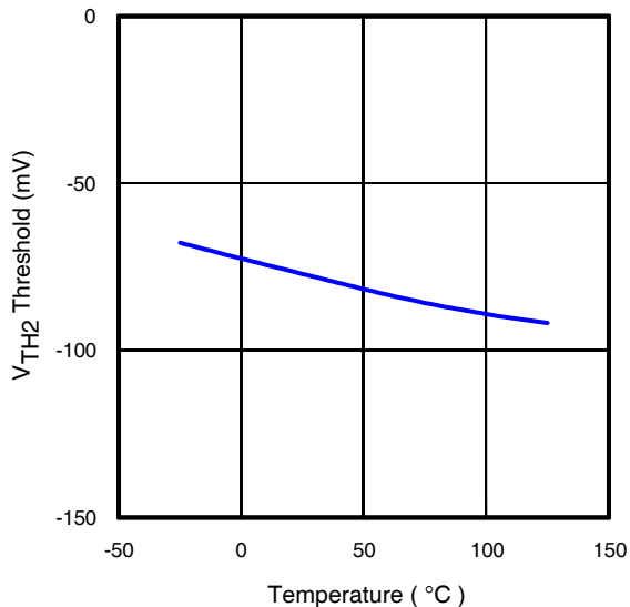
Fig 4. V_{\text{TH2}} vs. Temp.
