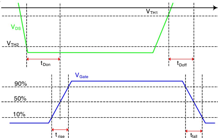
Fig. 15 - Timing Diagrams
