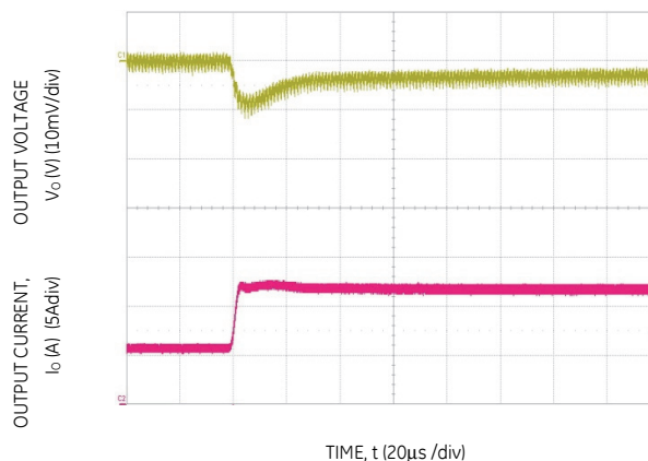
Figure 4. Transient Response to Dynamic Load Change from 50% to 100% at 12Vin, C_{out}=1 \times 47\mu\text{F}+11 \times 330\mu\text{F} , C_{Tune}=47\text{nF} , R_{Tune}=180\Omega
