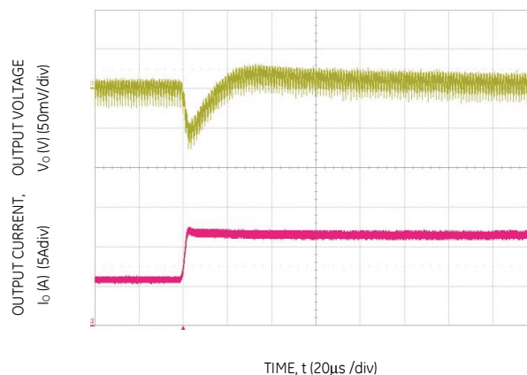
Figure 22. Transient Response to Dynamic Load Change from 50% to 100% at 12Vin, C_{out} = 2 \times 47\mu\text{F} + 1 \times 330\mu\text{F} , C_{Tune}=4700\text{pF} & R_{Tune}=240\Omega
