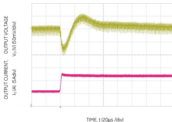
Figure 28. Transient Response to Dynamic Load Change from 50% to 100% at 12V in , C_{out} = 2 \times 47\mu\text{F} + 1 \times 330\mu\text{F} , C_{Tune}=2700\text{pF} & R_{Tune}=300\Omega
