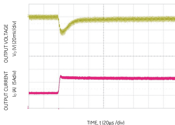
Figure 10. Transient Response to Dynamic Load Change from 50% to 100% at 12Vin, C_{out} = 3 \times 47\mu\text{F} + 3 \times 330\mu\text{F} , C_{Tune} = 12\text{nF} & R_{Tune} = 220\text{ ohms}
