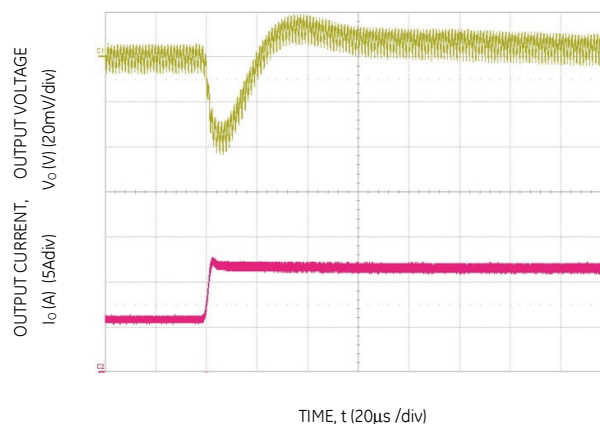
Figure 16. Transient Response to Dynamic Load Change from 50% to 100% at 12Vin, C_{out} = 2 \times 47\mu\text{F} + 2 \times 330\mu\text{F} , C_{Tune}=5600\text{pF} & R_{Tune}=220\Omega
