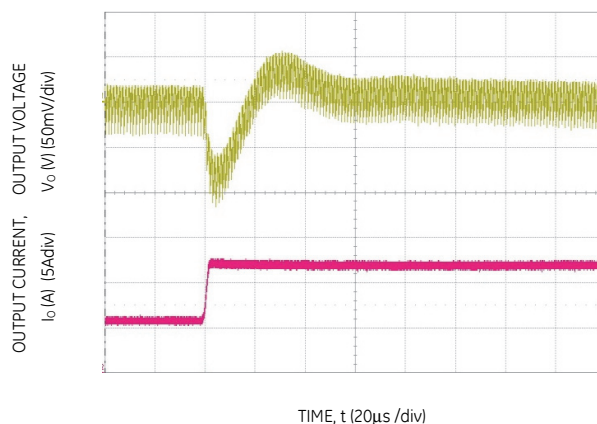
Figure 34. Transient Response to Dynamic Load Change from 50% to 100% at 12Vin, C_{out} = 1 \times 47\mu\text{F} + 1 \times 330\mu\text{F} , C_{Tune}=2200\text{pF} & R_{Tune}=300\Omega
