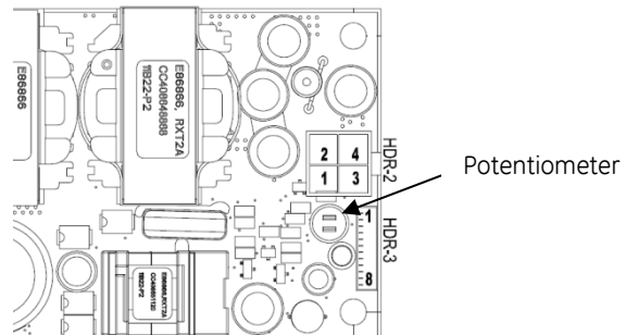
Fig. 10. Diagram showing location of the potentiometer used to adjust the power supply output voltage.
