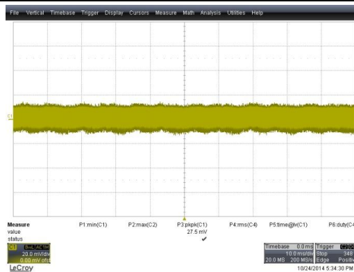
Figure 24. V_{OUT\_RIPPLE} = 27.5 \text{ mVp-p} , Output with 85 V AC and 50% Load Condition, (CH1: V OUT (20 mV AC /div), Time: 10 ms/div)
