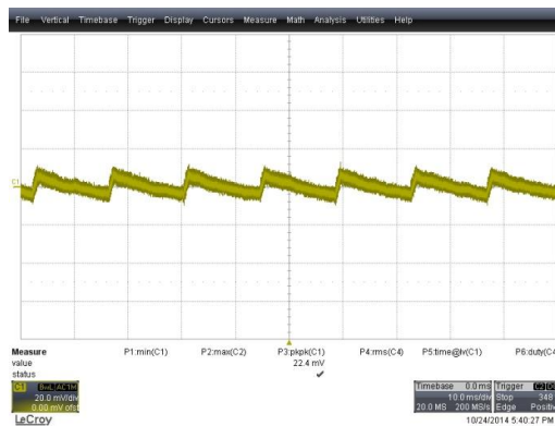
Figure 26. V_{OUT\_RIPPLE} = 22.4 \text{ mVp-p} , Output with 85 V AC and No-Load Condition, (CH1: V OUT (20 mV AC /div), Time: 10 ms/div)
