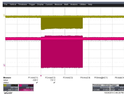
Figure 19. V_{DS}=731\text{ V} , V_{DIODE}=328\text{ V} , Output Short, Full-Load Condition, 460\text{ V}_{AC} , (CH1: V_{DIODE} (200 V/div), CH2: V_{DS} (200 V/div), Time: 50 ms/div)
