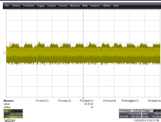
Figure 25. V_{OUT\_RIPPLE} = 42.9 \text{ mVp-p} , Output with 460 V AC and 50% Load Condition, (CH1: V OUT (20 mV AC /div), Time: 10 ms/div)
