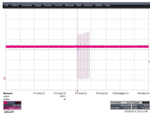
Figure 20. V_{DS}=936\text{ V} , Secondary Diode Short (AOCP), Full-Load Condition, 460\text{ V}_{AC} , (CH1: V_{DIODE} (200 V/div), CH2: V_{DS} (200 V/div), Time: 200 μs/div)
