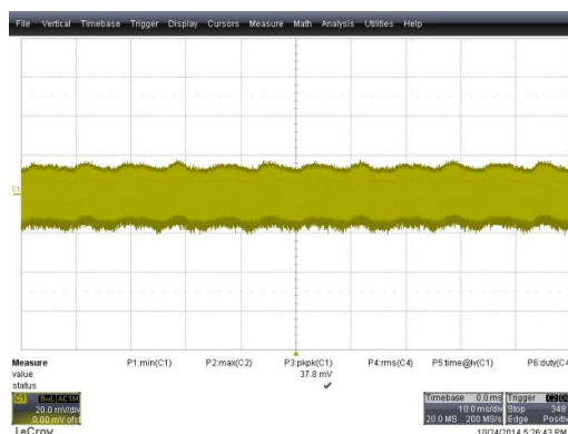
Figure 22. V_{OUT\_RIPPLE} = 37.8 mVp-p, Output with 85 V AC and Full-Load Condition, (CH1: V OUT (20 mV AC /div), Time: 10 ms/div)
