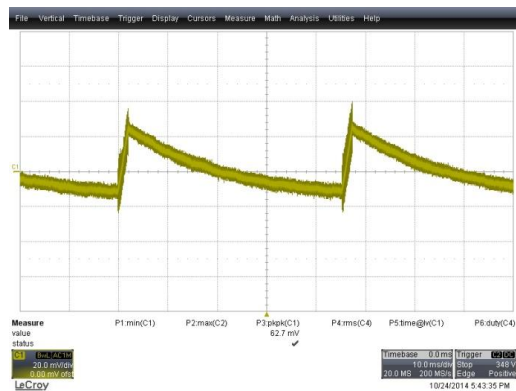
Figure 27. V_{OUT\_RIPPLE} = 62.7 \text{ mVp-p} , Output with 460 V AC and No-Load Condition, (CH1: V OUT (20 mV AC /div), Time: 10 ms/div)
