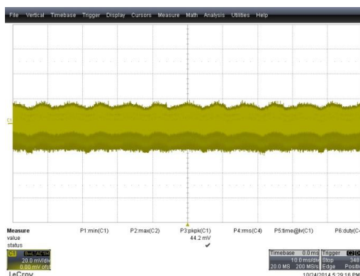
Figure 23. V_{OUT\_RIPPLE} = 44.2 mVp-p, Output with 460 V AC and Full-Load Condition, (CH1: V OUT (20 mV AC /div), Time: 10 ms/div)
