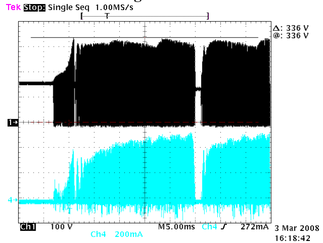
Ch1: V_{Drain} @ 100V/div, Ch4: I_{Drain} @ 200mA/div, time-base @ 5ms/div, V_{Drain(max)} = 336V
