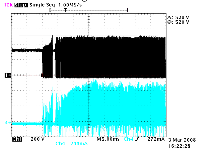
Ch1: V_{Drain} @ 200V/div, Ch4: I_{Drain} @ 200mA/div, time-base @ 5ms/div, V_{Drain(max)} = 520V
