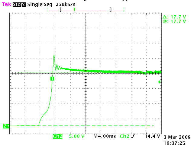
Ch2: V_{OUT} @ 5V/div, time-base @ 4ms/div
