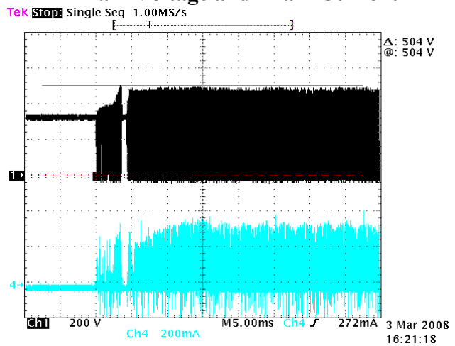
Ch1: V_{Drain} @ 200V/div, Ch4: I_{Drain} @ 200mA/div, time-base @ 5ms/div, V_{Drain(max)} = 504V
