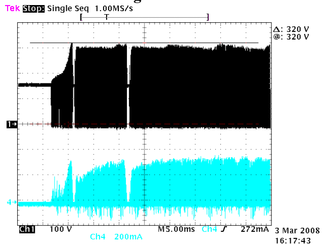
Ch1: V_{Drain} @ 100V/div, Ch4: I_{Drain} @ 200mA/div, time-base @ 5ms/div, V_{Drain(max)} = 320V
